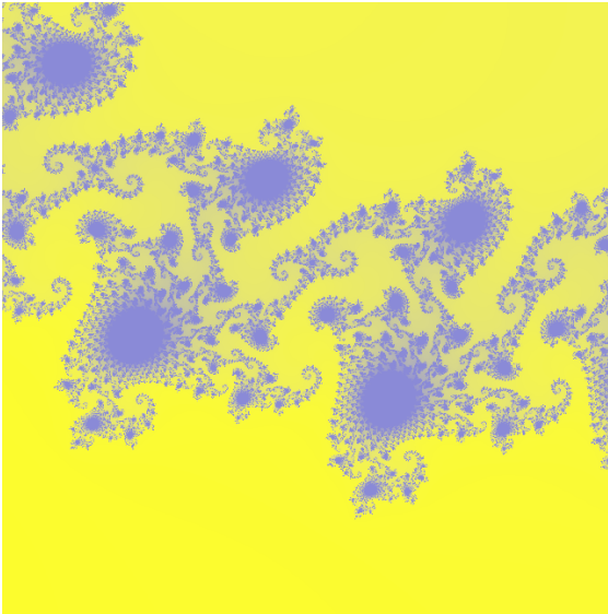
Illustration 1: ./mandelbrot -0.74364990 0.13188204 0.00073801 image.png
