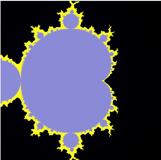
Illustration 3: ./mandelbrot 0.0 0.0 2.0 image2.png
