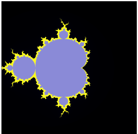
Illustration 4: ./mandelbrot 0.0 0.0 3.0 image3.png
