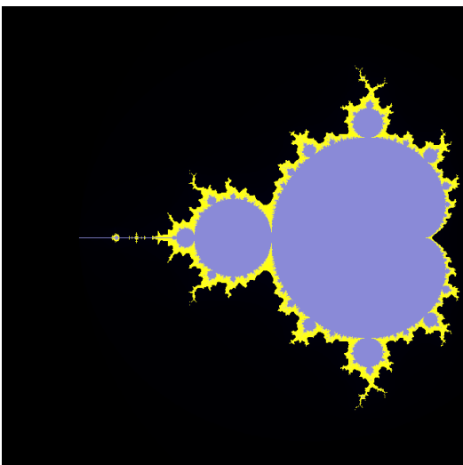
Illustration 5: ./mandelbrot -1.0 0.0 3.0 image3-1.png
