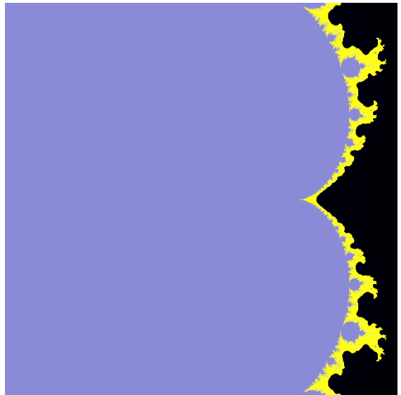
Illustration 2: ./mandelbrot 0.0 0.0 1.0 image1.png
